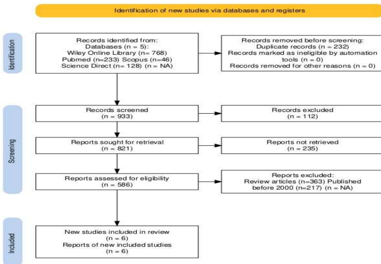
Figure 1: PRISMA Flowchart
